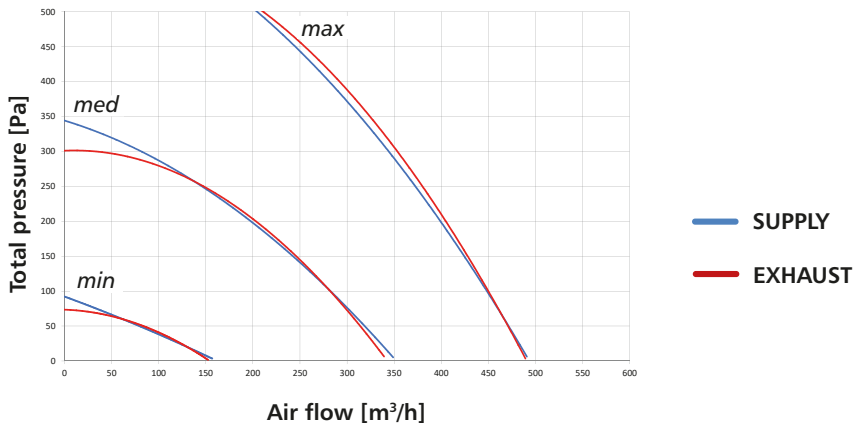
Air flow HRU-PremAir-450 / HRU-PremAir-450E
