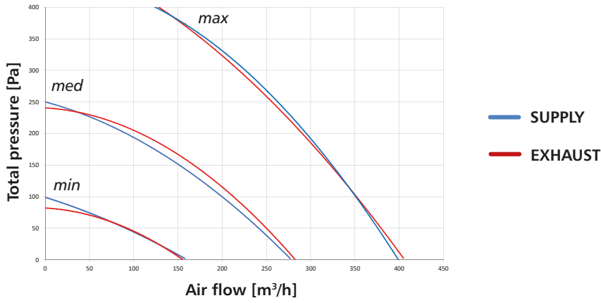
Air flow HRU-PremAir-350 / HRU-PremAir-350E
