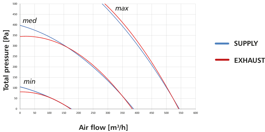
Air flow HRU-PremAir-500
